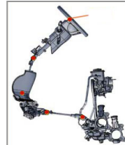
Energy absorbing type steering column
